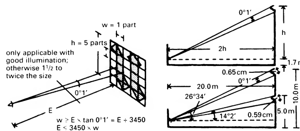
⑥ To be readable at a distance of, say, 700m the width w of the letters must be: \geq 700 \times 0.000291 = 0.204 ; height h is usually 5w: 5 \times 0.204 = 1.020m ⑦ As in the previous examples, the size of structural parts which are differentiable can be calculated using the viewing distance and trigonometry
